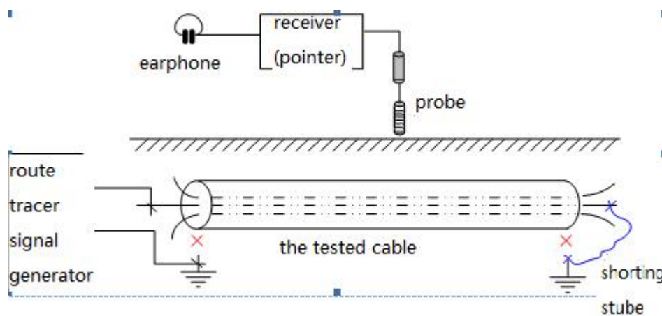
Special route detection wiring diagram.
