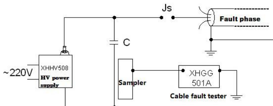
Graph 2:Inductive sampling connection
